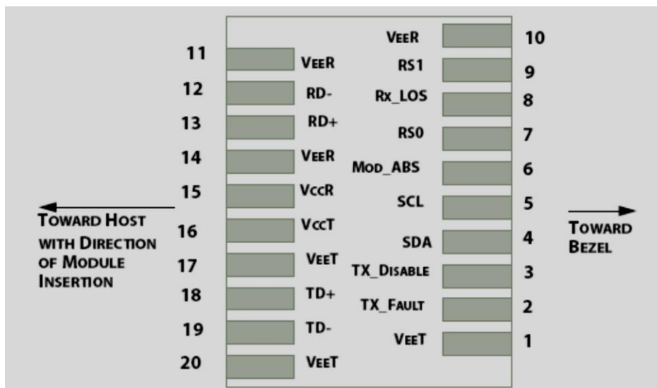
Figure 4: Module Interface to Host
