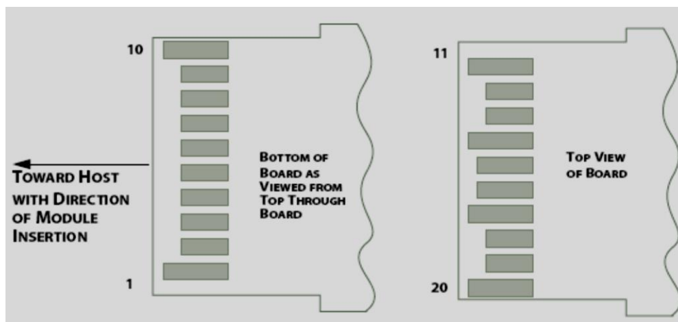
Figure 5: Module Contact Assignment
