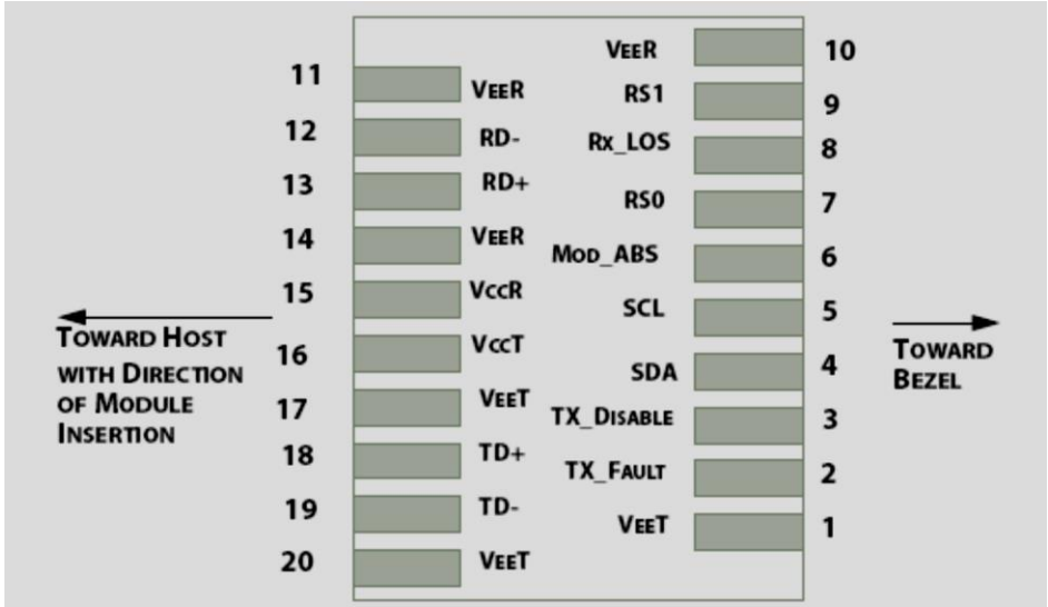
Figure 3: Module Interface to Host
